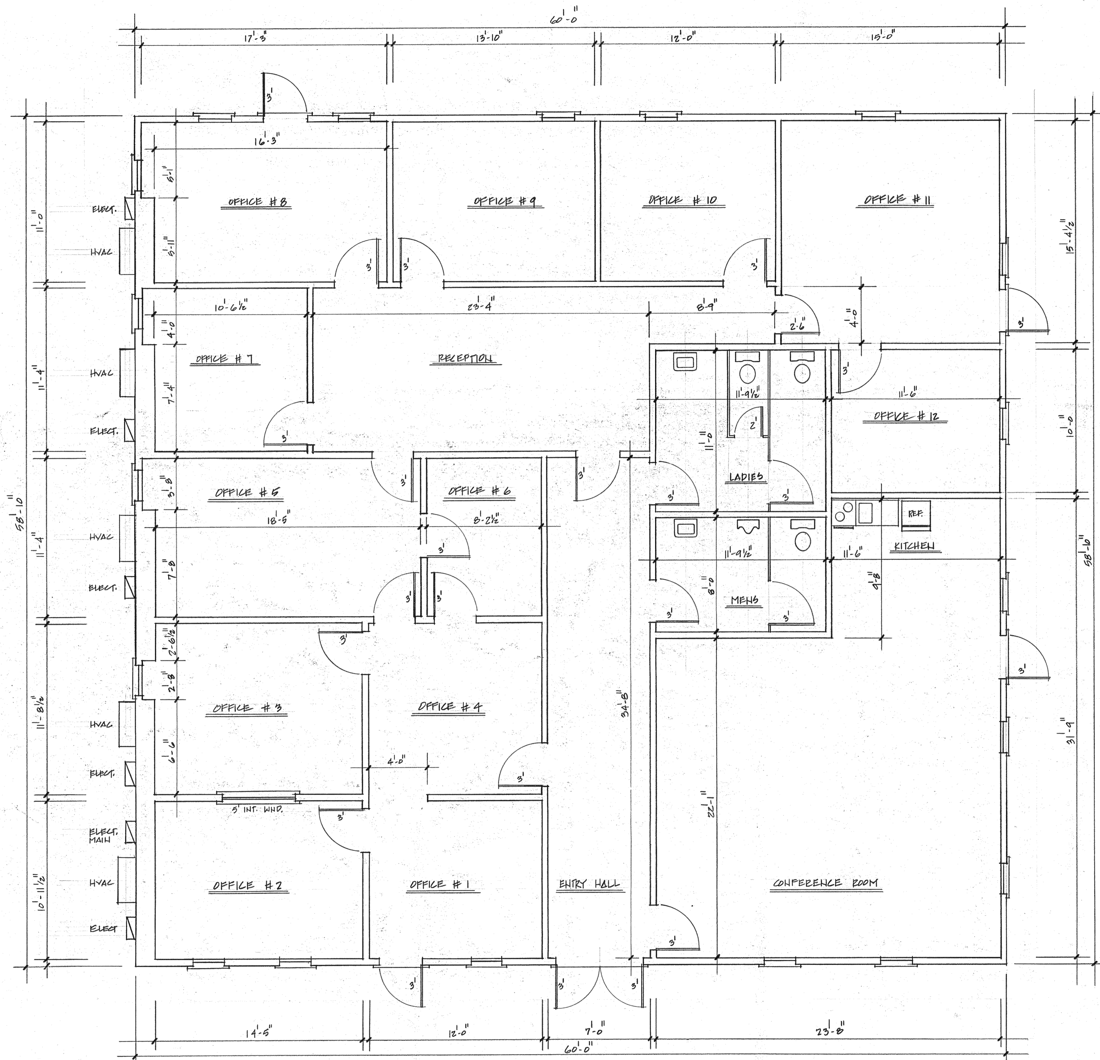
BUILDING "D" PLAN, AS-BUILT
