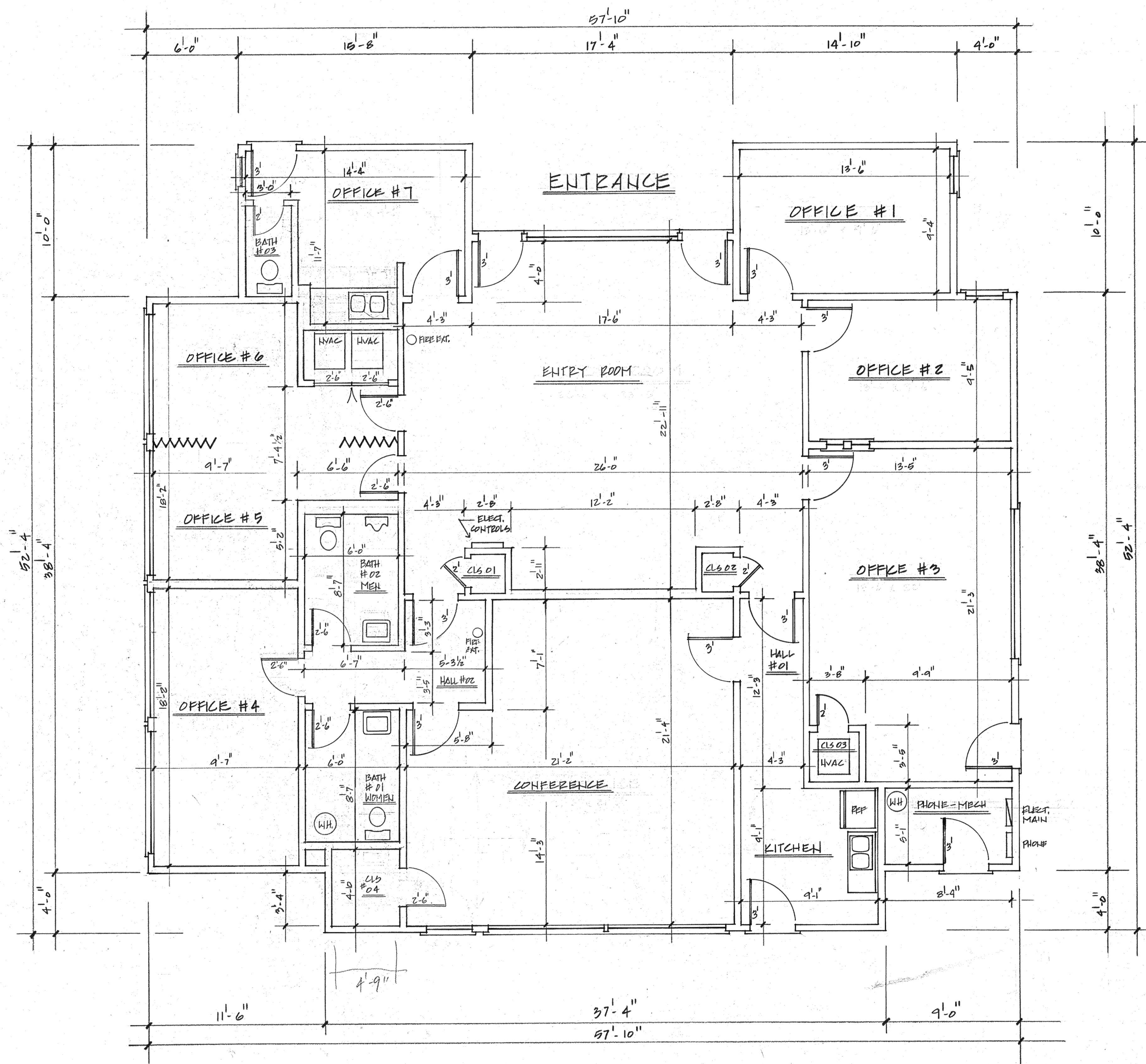
BUILDING "B" PLAN, AS-BUILT 1/4" = 1'-0"
